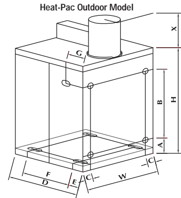
Sealed System Option Available Up to 150,000 Btu's
